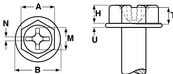
PHILLIPS HEX WASHER HEADS FOR MACHINE SCREWS
