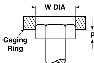
SLOTTED HEX WASHER HEADS WITH SERRATIONS FOR MACHINE SCREWS
