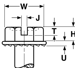
SLOTTED HEX WASHER HEADS WITH SERRATIONS FOR MACHINE SCREWS
