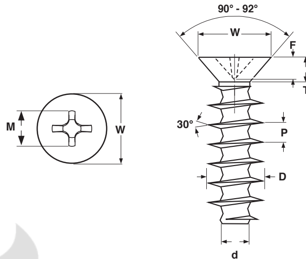
METRIC - TYPE PT®-ALTERNATIVE THREAD FORMING SCREWS, FLAT PHILLIPS
