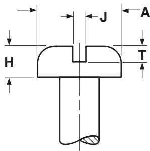
PAN HEADS FOR SELF-TAPPING AND DRILLING SCREWS
