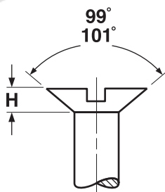
FLAT HEAD 100° FOR SELF-TAPPING SCREWS
