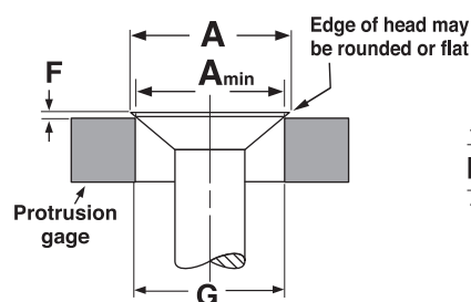
FLAT HEAD 100° FOR SELF-TAPPING SCREWS
